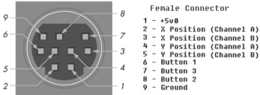
Figure 8-3: The Bus Mouse Pins
